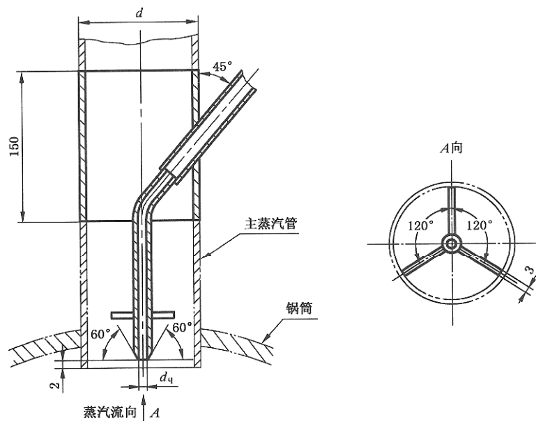
图 C.1 饱和蒸汽取样头
