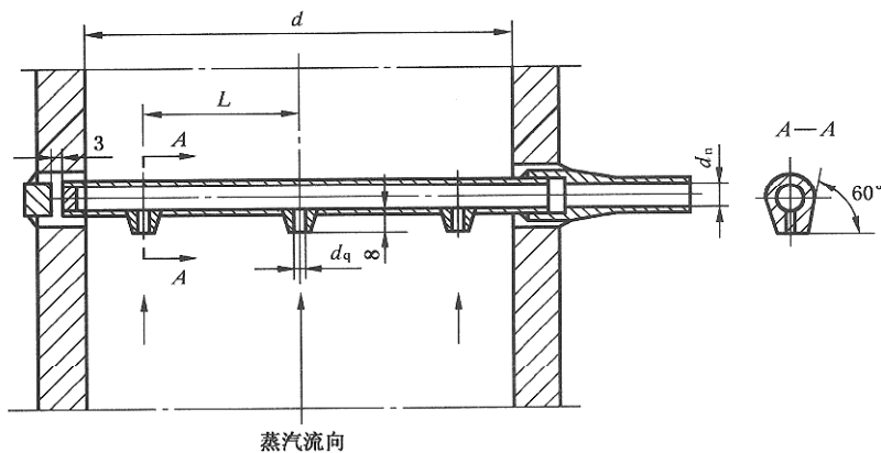
图 C.1 饱和蒸汽取样头
